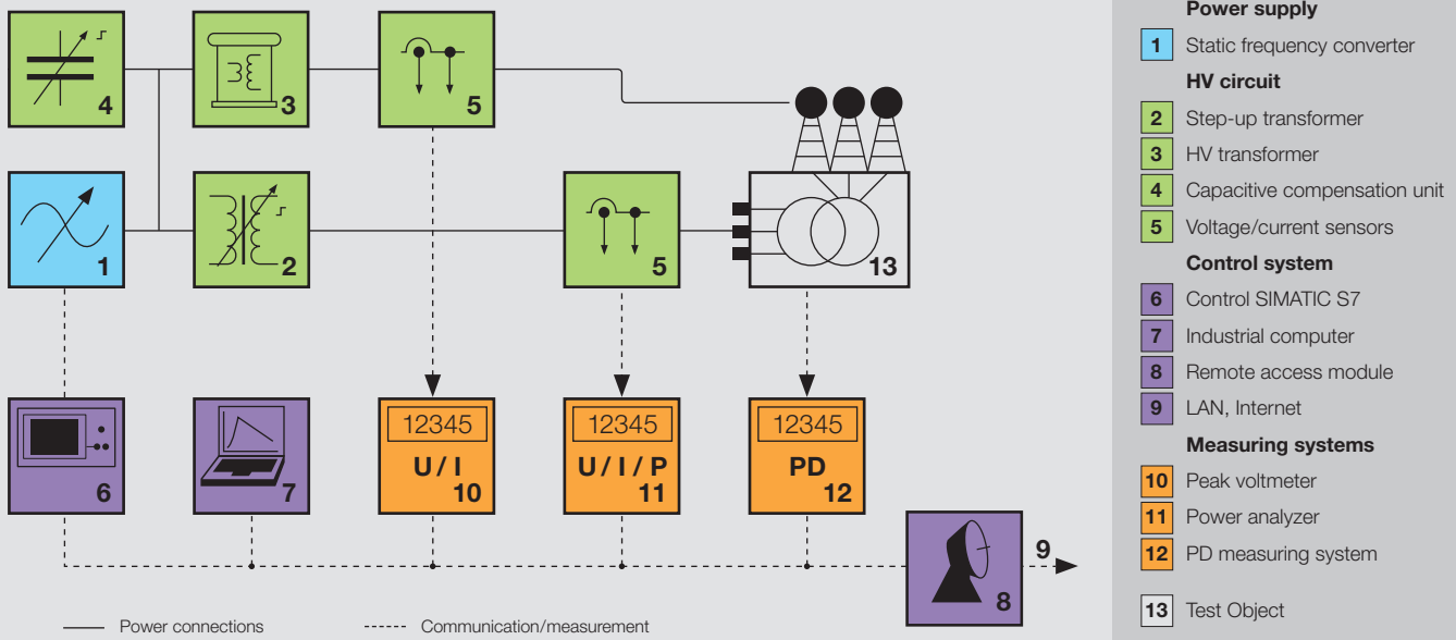
Fig. 3 Block diagram for factory testing of transformers
